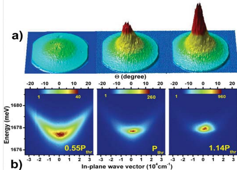
Momentum distribution
