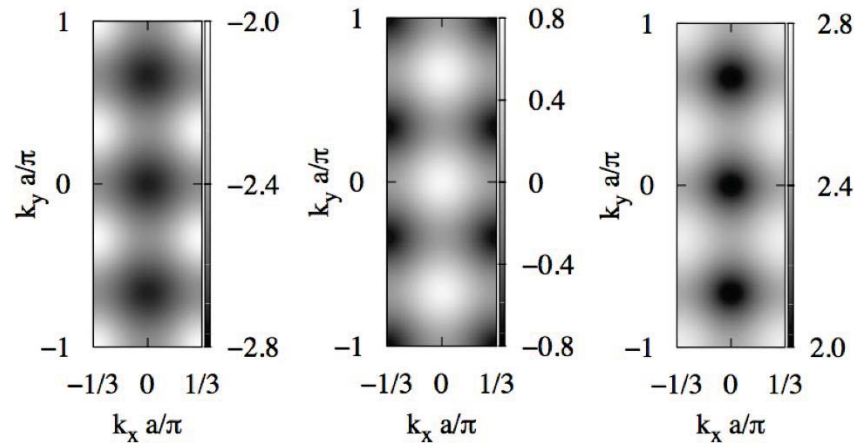
Band dispersion
