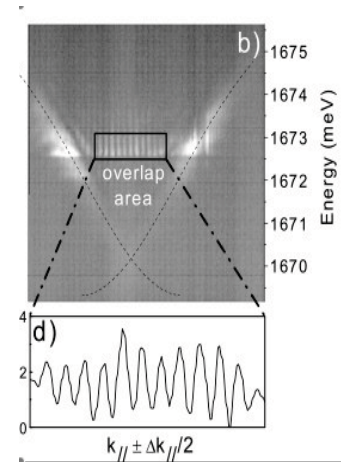
Interference
