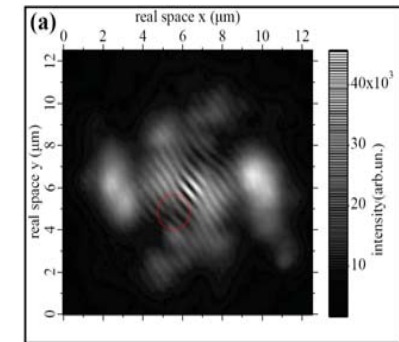
Quantized vortices
