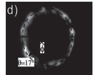
BEC on k-space ring
